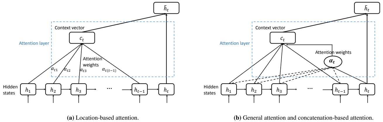
Figure 3: Attention mechanisms.
